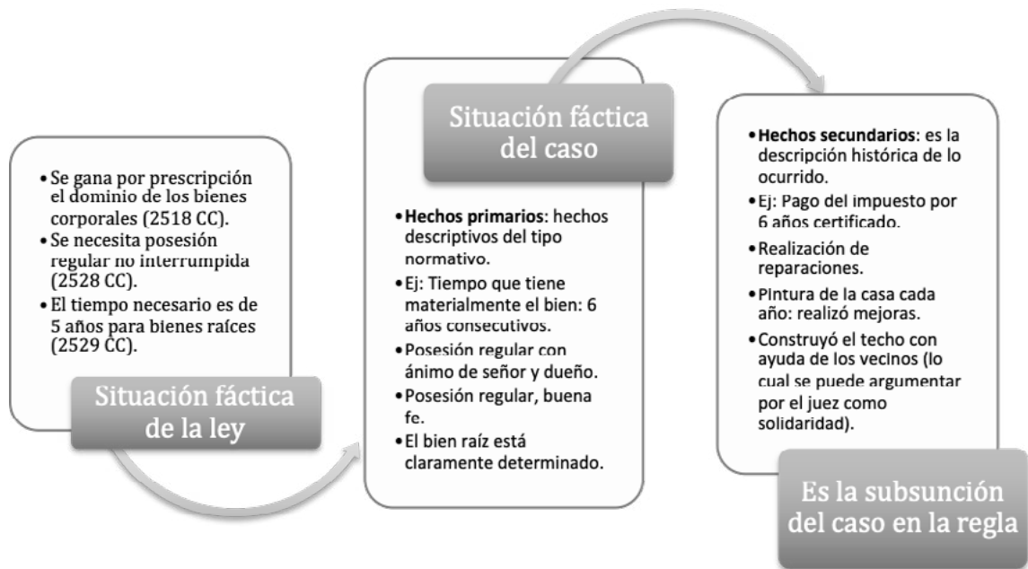
Figura 1. Premisa mayor
